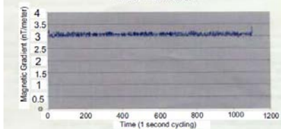
Sample data Gradiometer data shows very low noise level (<0.2nT. peak to peak)
